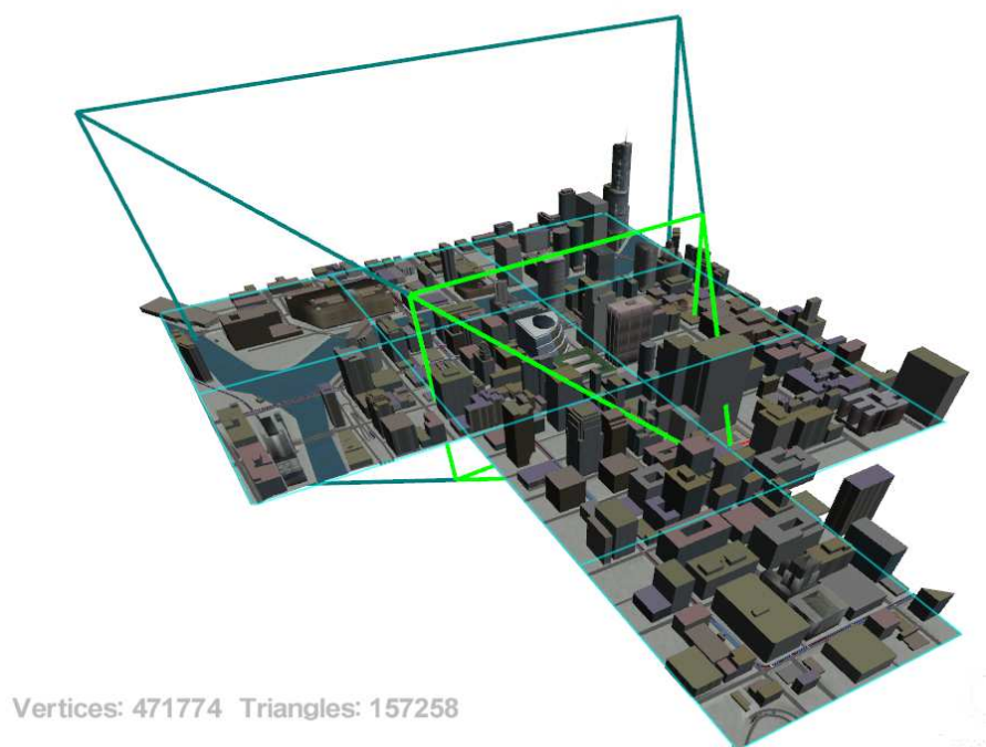
Figure 2 City tiles intersecting the view frustum
